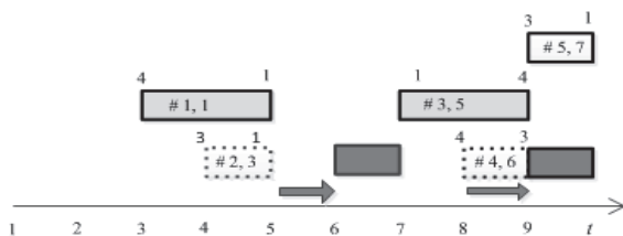
Figure 2: Diagram of execution of adaptive schedule by one truck.
